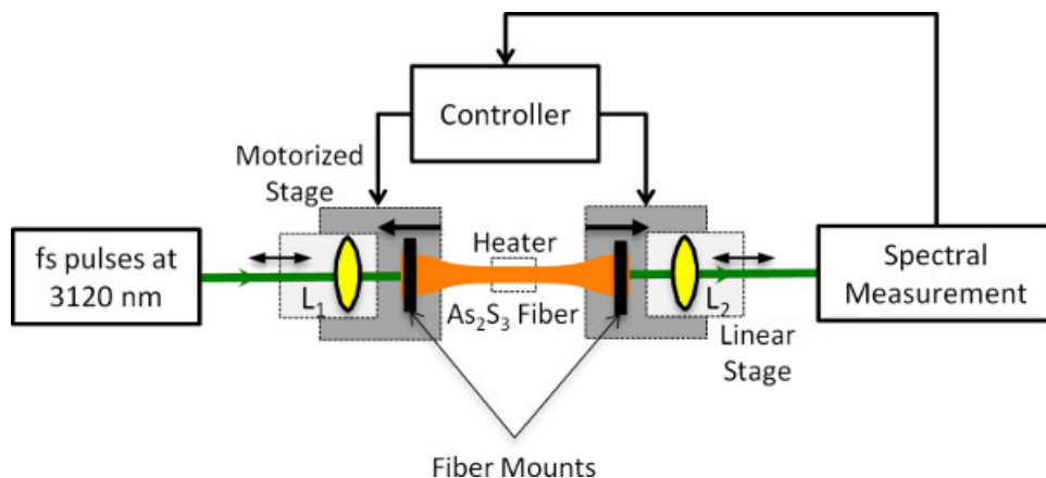
Figure 1. In-situ Fiber Tapering Setup. The fs pump source is coupled into the As_2S_3 fiber with lens L_1 by optimizing L_1 's linear stage position (shown in light gray) and the XY position of the lens mount (not shown in the figure). The output of the fiber is coupled to the spectral measurement device with L_2 optimized by a linear stage. The motorized stages (shown in dark gray) pull the fiber away from the central heater and stop when the spectral measurement value is maximized.
