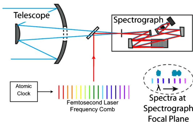
Fig. 6. (Color online) Concept of an astronomical spectrograph calibrated by a femtosecond laser frequency comb. The atomically-referenced comb spectrum enters the spectrograph offset from the star light such that it appears below the dispersed stellar spectrum. In reality a fiber-fed spectrograph is preferable to reduce pointing errors. The optimum spacing of the comb lines is one every 3–4 resolution elements [86], amounting to \sim 30 \text{ GHz} for a visible spectrograph with resolving power of 60,000.
