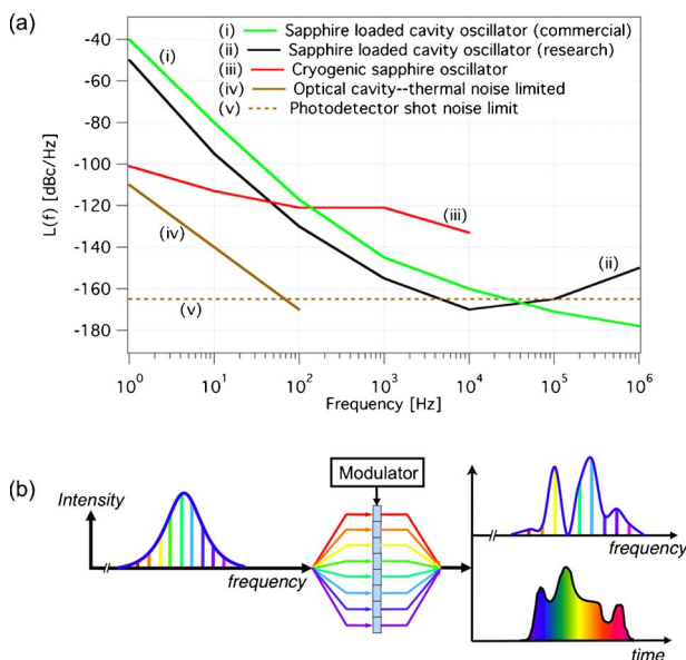
Fig. 7. (Color online) (a) Comparison of measured and projected phase noise on the 10 GHz signal generated from a few sources. (i) measured commercial sapphire oscillator [94], (ii) measured research sapphire oscillator [95], (iii) measured cryogenic sapphire oscillator [96], (iv) projected phase noise for a frequency comb locked to a cw laser that is stabilized to a high-finesse reference cavity [97,98,100]. (v) dashed line is the projected white noise floor given by photodetector shot noise. (b) General approach to line-by-line pulse shaping with an optical frequency comb. The different comb elements are spatially/spectrally dispersed and directed to a modulator array, where individual comb lines are modified in amplitude and phase. The modes are then re-combined to form an optical field with user-defined spectral and temporal characteristics.
