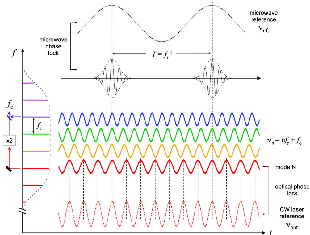
Fig. 2. (Color online) Time-frequency interpretation of the output of the mode-locked laser. The frequency modes \nu_n = n \cdot f_r + f_0 of the mode-locked laser are essentially a series of cw oscillators tightly locked in phase that coherently add to form a short pulse at a period T , which is the inverse of the repetition rate. The carrier-envelope offset frequency f_0 is measured via the heterodyne between the second harmonic ( \times 2 ) of the infrared and visible comb components. For simplicity, f_0 is shown with the value of zero, such that every pulse is identical. The repetition rate (mode spacing) f_r can be measured with a fast photodiode and compared or phase-locked to a microwave reference \nu_{r,f} . Alternatively, mode N of the comb can be heterodyned with an external cw laser at frequency \nu_{opt} . Active feedback to the frequency comb can force the comb mode to oscillate in phase with the cw laser, and as the other modes are already locked in phase via the mode-locking mechanism, f_r assumes the value of f_r = (\nu_{opt} + f_0)/N .
