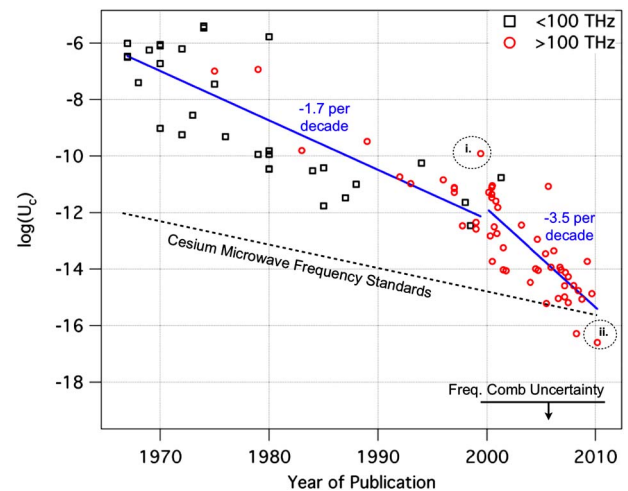
Fig. 4. (Color online) Record of improvement of precise frequency measurements in the optical and terahertz domains over time. The y-axis is the base-ten logarithm of the fractional uncertainty U_c = \sigma/\nu_0 , where \sigma is the standard uncertainty and \nu_0 is the carrier frequency. A distinction is made between frequencies less than and greater than 100 THz, which is somewhat arbitrarily defined as the beginning of the “optical” domain. Note that there were just a few measurements at frequencies greater than 100 THz prior to 1990, and it was not until the introduction of the femtosecond laser frequency comb around 2000 that the rate at which optical frequencies were measured truly accelerated and became commonplace. The circled points are a few noteworthy measurements: (i) The first measurement of an optical frequency involving a femtosecond laser frequency comb [55]. (ii) The most accurate measurement of an optical frequency standard, which is presently the ratio of the frequencies of two \text{Al}^+ quantum logic clocks with combined uncertainty of 2.5 \times 10^{-17} . The evaluated inaccuracy of one of the \text{Al}^+ clocks is a factor of \sim 3 smaller at 8.6 \times 10^{-18} [63]. The residual fractional uncertainty of the frequency comb in the comparison of optical frequency standards and the construction of an optical clock is at or below 1 \times 10^{-19} .
