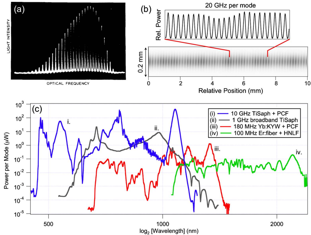
Fig. 3. (Color online) Spectra of early and more recent frequency combs. (a) Spectrum of first mode-locked laser operating near 633 nm, as measured with a scanning Fabry-Perot etalon. The mode spacing is \sim 56 MHz. Reprinted with permission from L. E. Hargrove, R. L. Fork, and M. A. Pollack, Appl. Phys. Lett. 5 , p. 4-5. Copyright 1964, American Institute of Physics. (b) A portion of the 20 GHz frequency comb generated by mode-filtering the output of a frequency-stabilized 1 GHz frequency comb [38]. The lower part of the figure is the grey-scale “fringes” of the comb as recorded with a grating spectrometer and CCD camera. The upper part of the figure shows a line out of a portion of the CCD image. The modes are spectrally separated by 20 GHz and spatially dispersed by about 100 microns per mode. Central wavelength is 960 nm. (c) Spectral envelope of some common optical frequency combs generated with different laser sources. (i) 10 GHz Ti:Saph [39], (ii) 1 GHz broadband Ti:Saph [37], (iii) 180 MHz Yb:KYW [26], (iv) 100 MHz Er:fiber [20].
