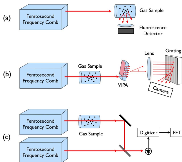
Fig. 5. (Color online) Three different spectroscopy approaches using femtosecond laser frequency combs. (a) Fluorescence detection. (b) Spectrally dispersed detection with a high resolution imaging spectrometer based on a VIPA (virtually-imaged phased array) disperser. (c) Dual comb multi-heterodyne spectroscopy with a point detector and high-speed data acquisition. In all cases, what is depicted as a vapor cell could in fact be atoms or molecules in a beam, trap, or other gas phase sample. In principle, liquids and solids could also be studied in a similar fashion.
